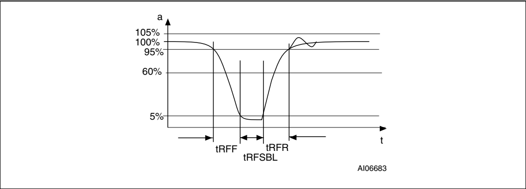
Figure 2. 100% modulation waveform
